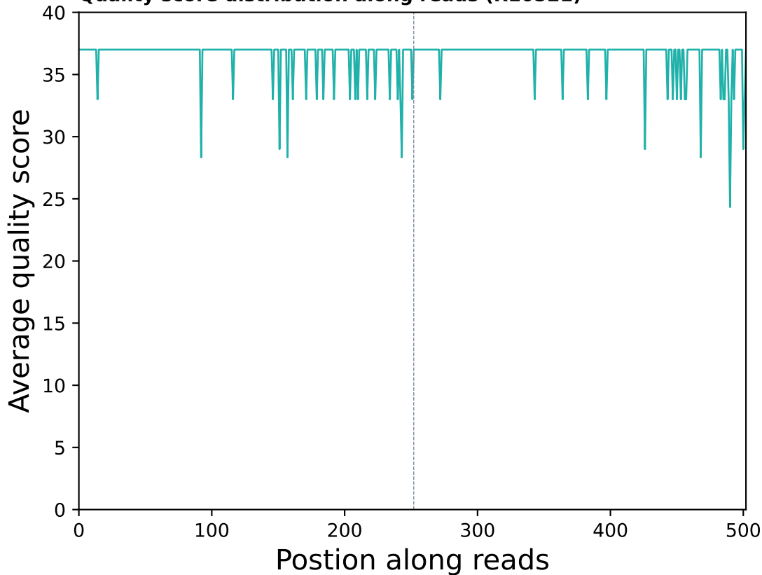
Quality score distribution along reads (R10521)
